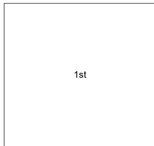
Drawings of the Observations of a Transit of Venus
